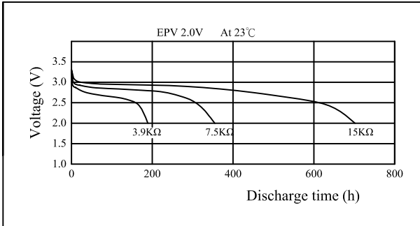
Discharge characteristics
