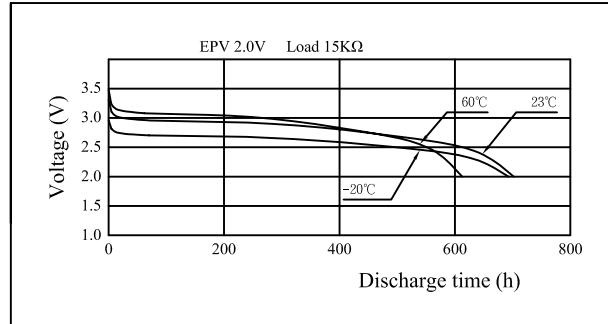
Temperature characteristics
